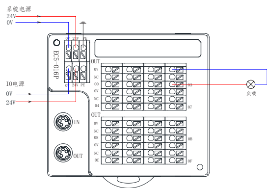
EC5-O16P (PNP输出)
