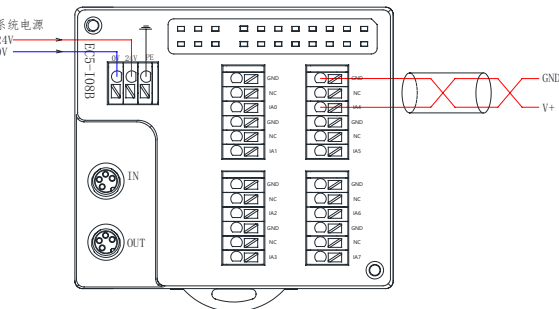
EC5-I08B (电压输入)
