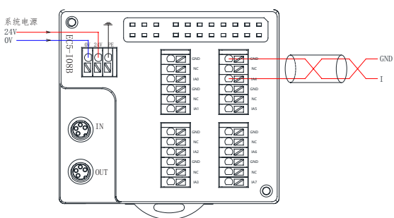
EC5-I08B (电流输入)
