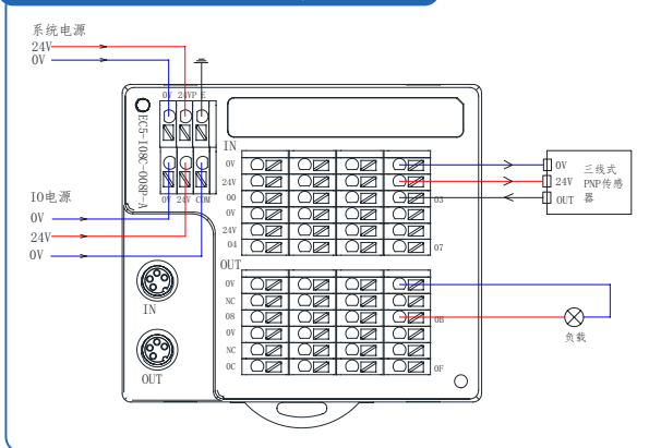
EC5-I08C-008P-A (PNP输入,PNP输出)
