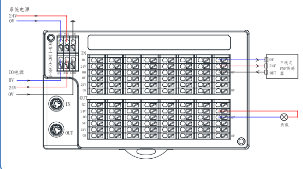
EC5-I16C-O16P-A (PNP输入,PNP输出)
